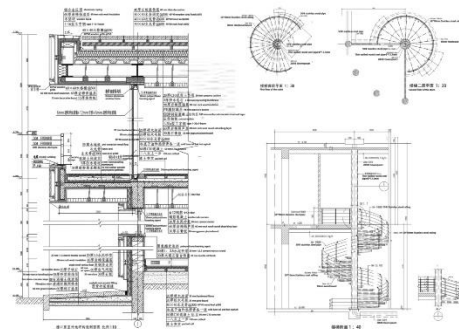
Figure 4 An example of structural construction design course integration (Source: Tsinghua University School of Architecture, Tsinghua University)
